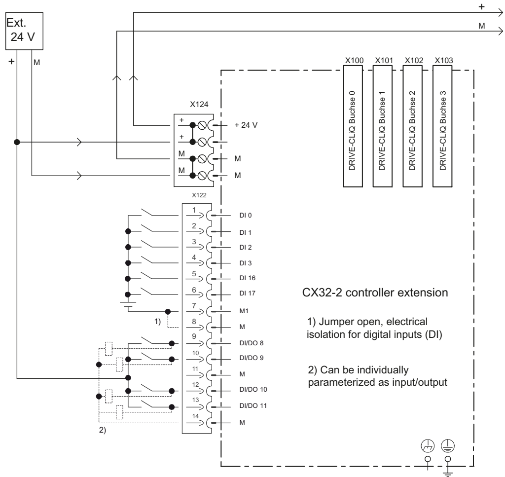
Figure 7-11 Digital I/Os connection diagram
