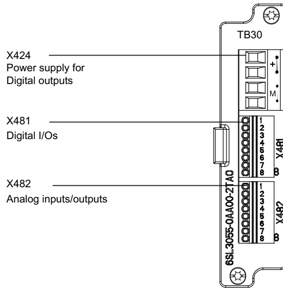
Figure 7-3 Interface arrangement on the TB30
