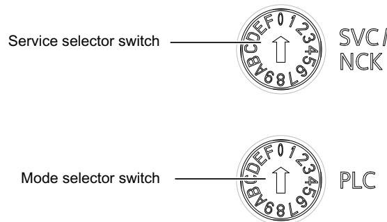
Figure 3-3 Selector switches for service and operating modes of the SIMOTION D4x5-2
