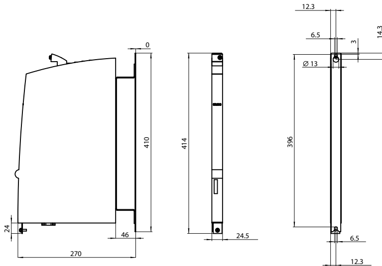
Figure 7-12 CX32-2 dimension drawings (dimensions in mm)
