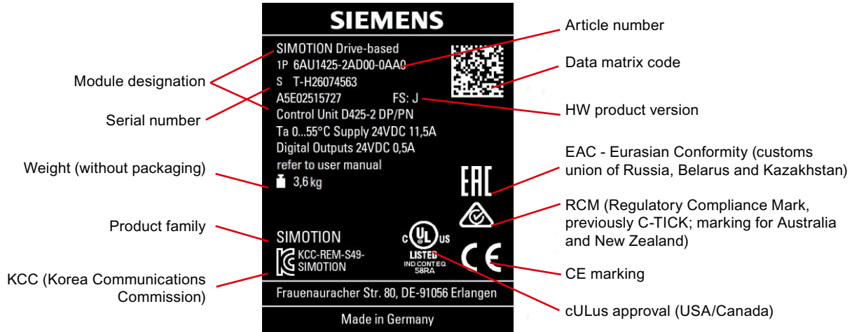
Figure 2-5 Rating plate using the D425-2 DP/PN as an example
