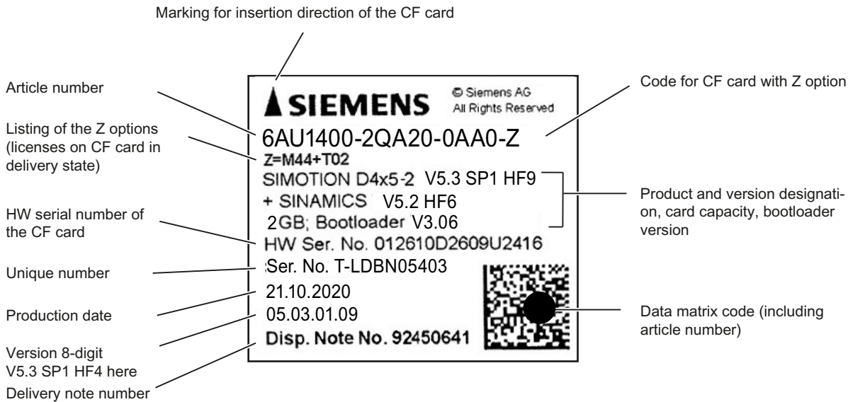
Figure 2-8 Rating plate of the CF card (example of 2 GB CF card)
