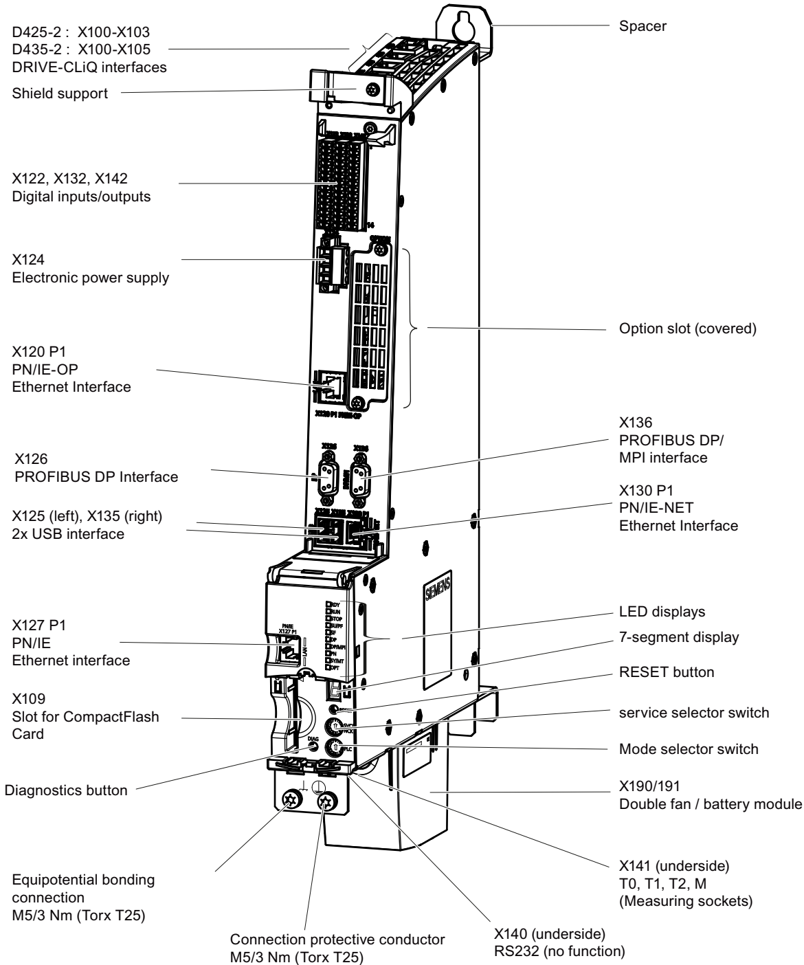
Figure 2-2 D425-2 DP and D435-2 DP representation
