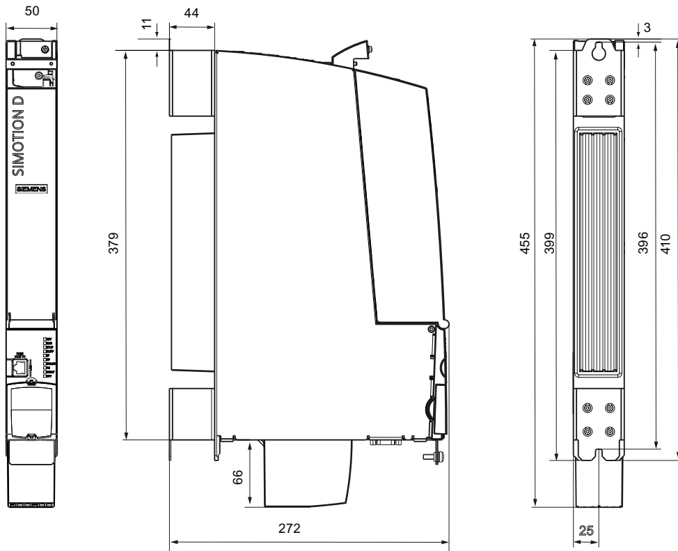
Figure 6-2 D445-2 DP/PN and D455-2 DP/PN dimension drawing (dimensions in mm)
