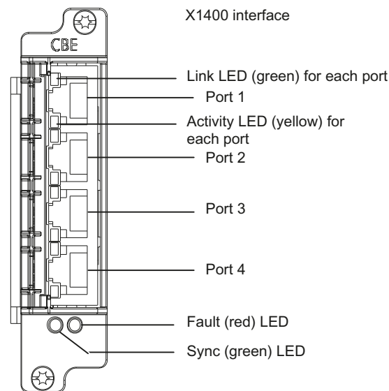
Figure 7-5 CBE30-2 front view
