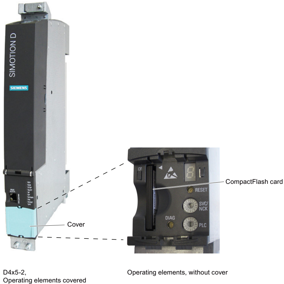
Figure 2-7 Slot for CompactFlash card
