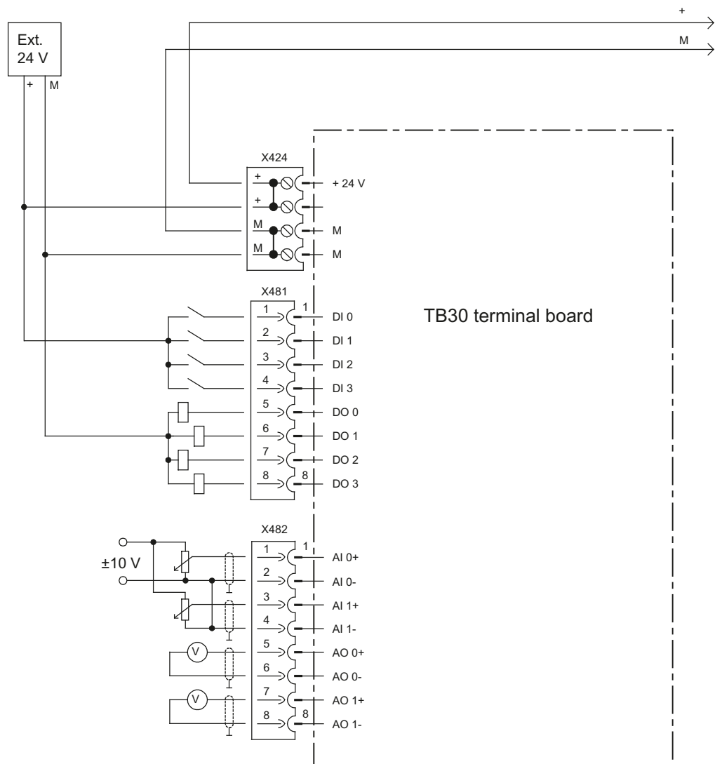
Figure 7-4 TB30 connection diagram
