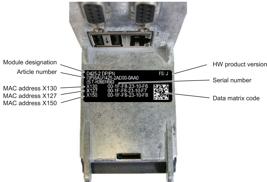
Figure 2-6 MAC addresses of SIMOTION D425-2 DP/PN
