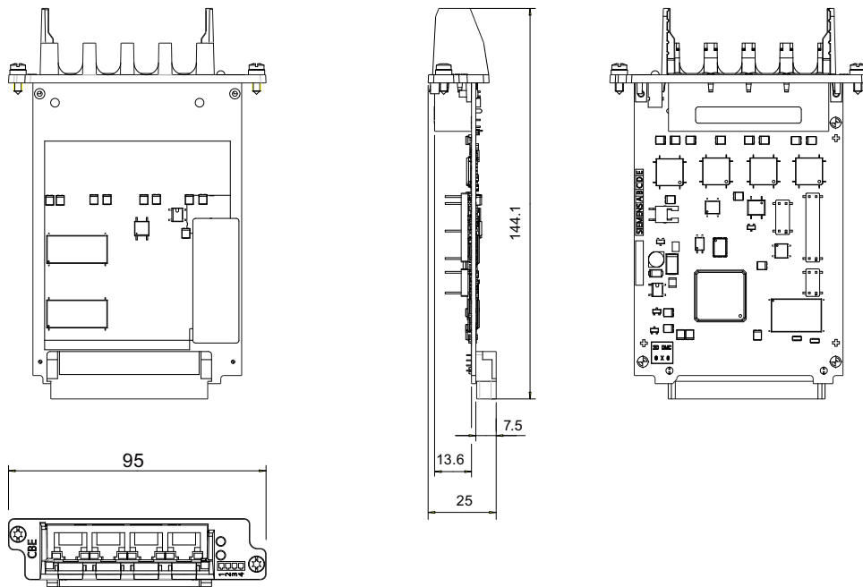
Figure 7-9 CBE30-2 dimension drawing (dimensions in mm)
