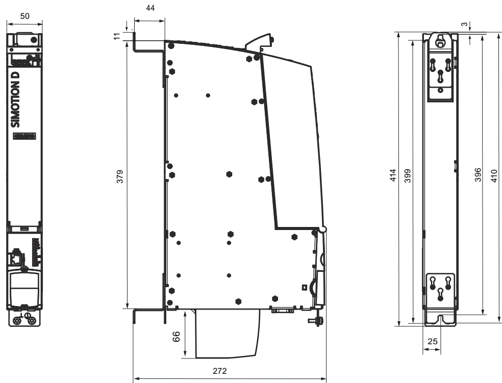
Figure 6-1 D425-2 and D435-2 dimension drawing (dimensions in mm)
