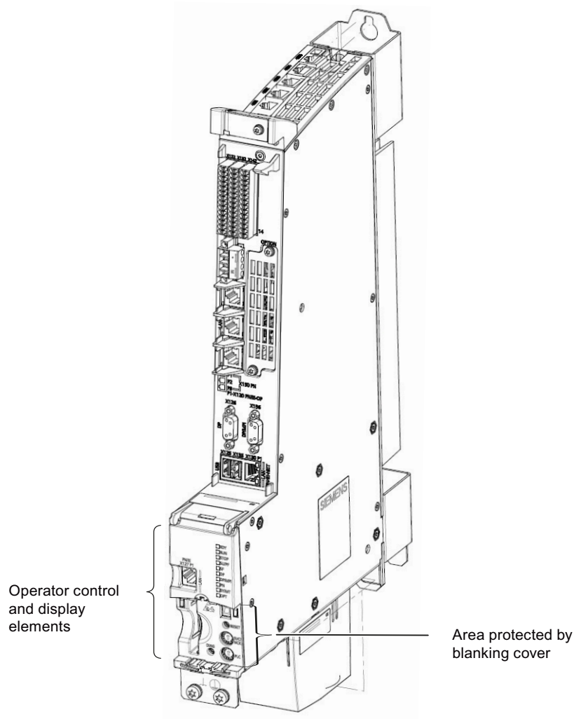
Figure 3-1 Position of operator control and display elements (example of SIMOTION D445-2 DP/PN)
