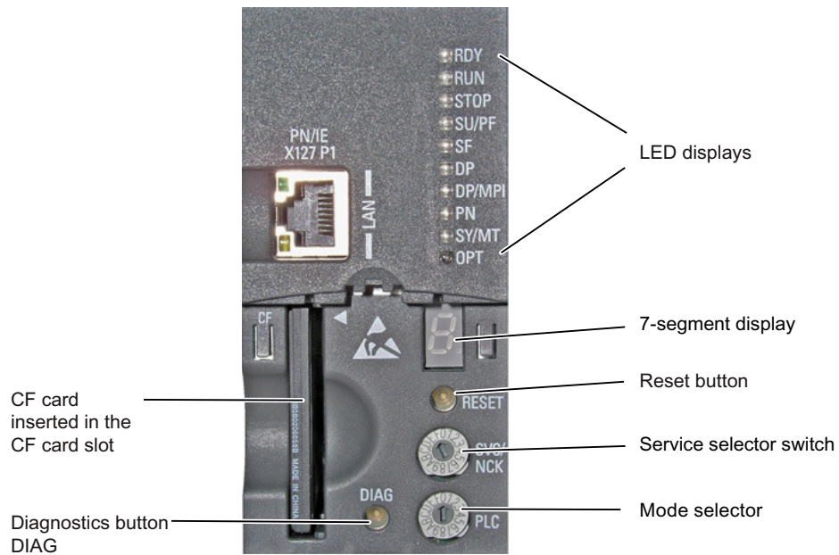
Figure 3-2 Control and display elements of the SIMOTION D4x5-2
