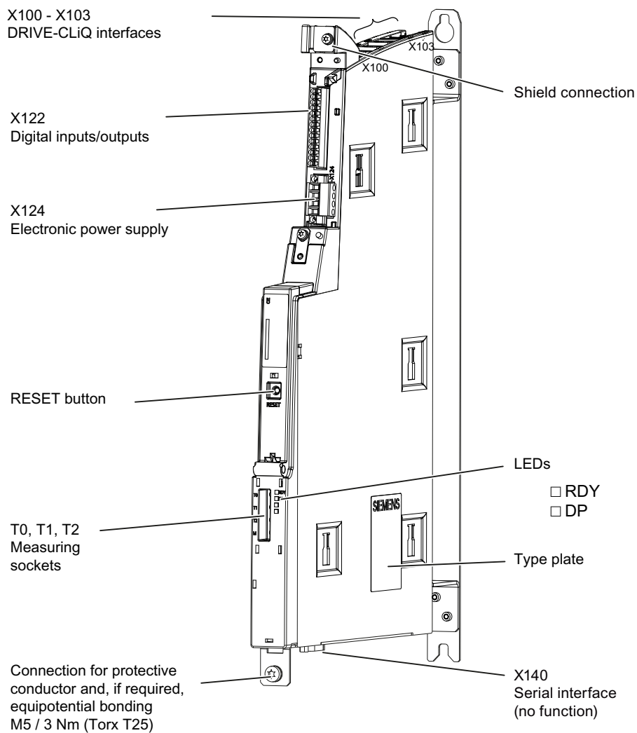
Figure 7-10 CX32-2 (without cover) with interfaces and operator control
