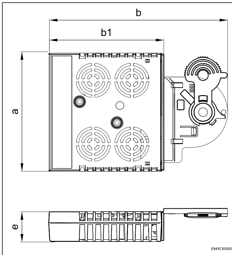
[4-2] Dimensions
