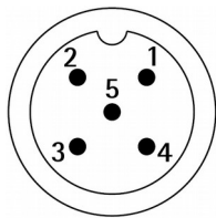
M12 5-pin male connector (frontal side)
