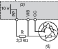
(2) ATV 212 control terminals (3) Motor
