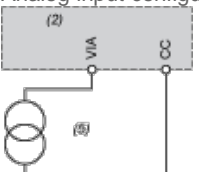
(2) ATV 212 control terminals (5) Source 0-20 mA, 4-20 mA, X-Y mA
