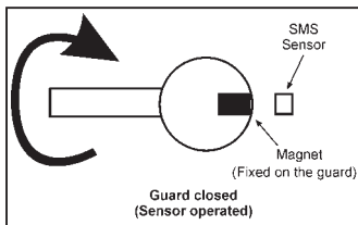
Fig. 6: Example of application on hinged guard
