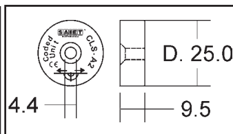
Fig. 3: CLS-A2 magnetic unit dimensions
