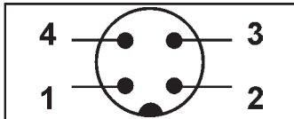
Fig. 8: Pin-out of male connectors
