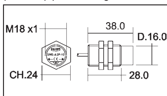
Fig. 2: Dim. of std cylindrical SMS (other available on request)
