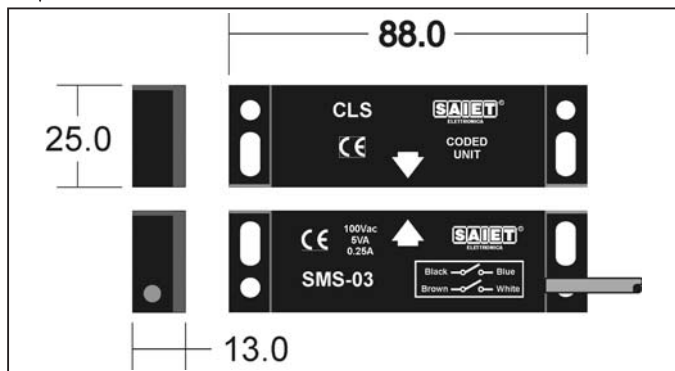
Fig. 1: Mechanical dimensions of the sensors and the operating units parallelepiped housing.
