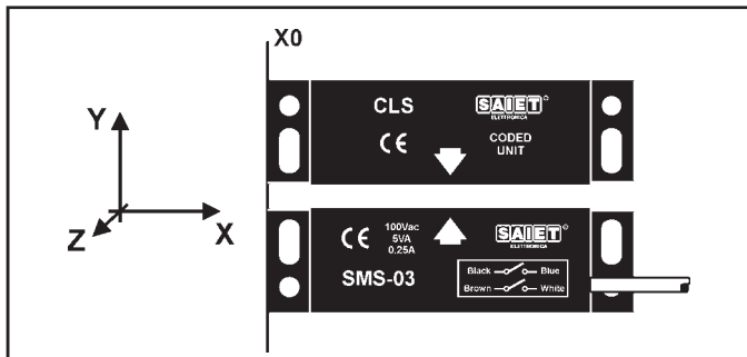
Fig. 4 - Operating and alignment direction of the parallelepiped sensors.
