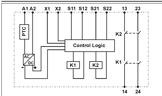
Fig. 1 - NA12D diagram
