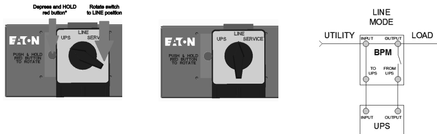
Figure 19. From UPS to LINE
