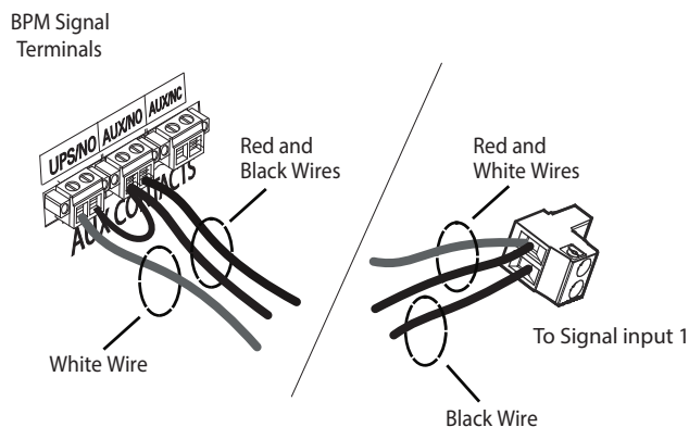
One Connector Option
