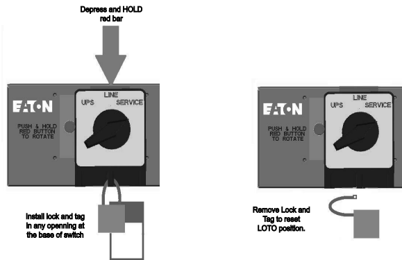
Figure 21. LOTO Feature
