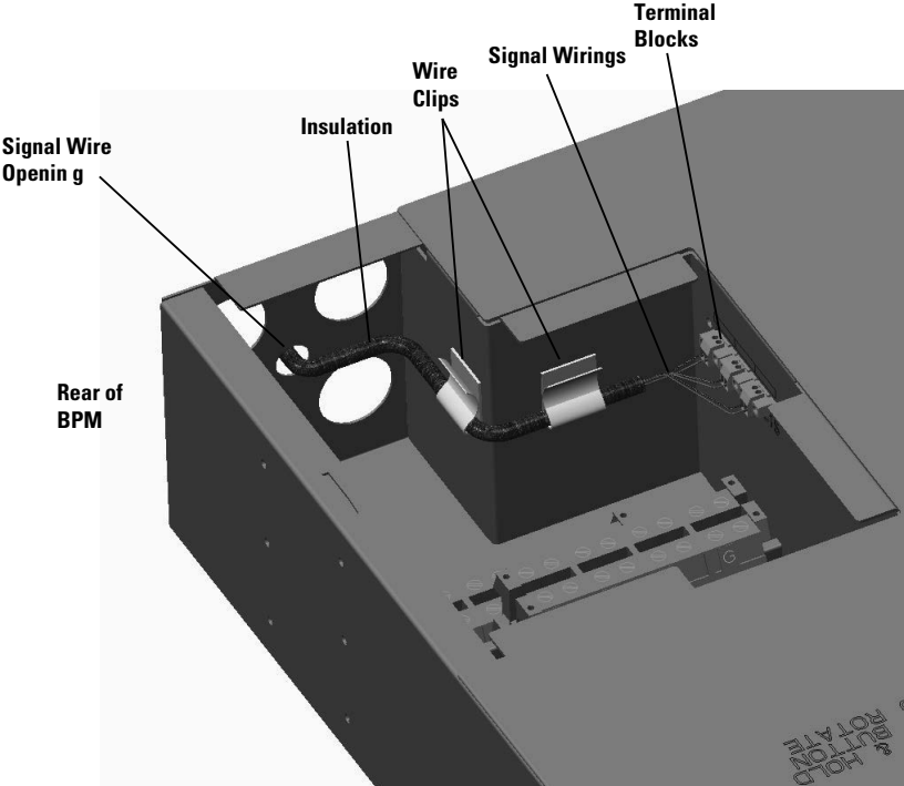
Figure 15. Signal Wire Routing
