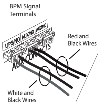
Two Connector Option
