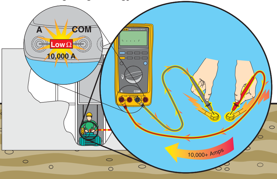
Figure 3. Misuse of DMM in Ammeter Mode.
