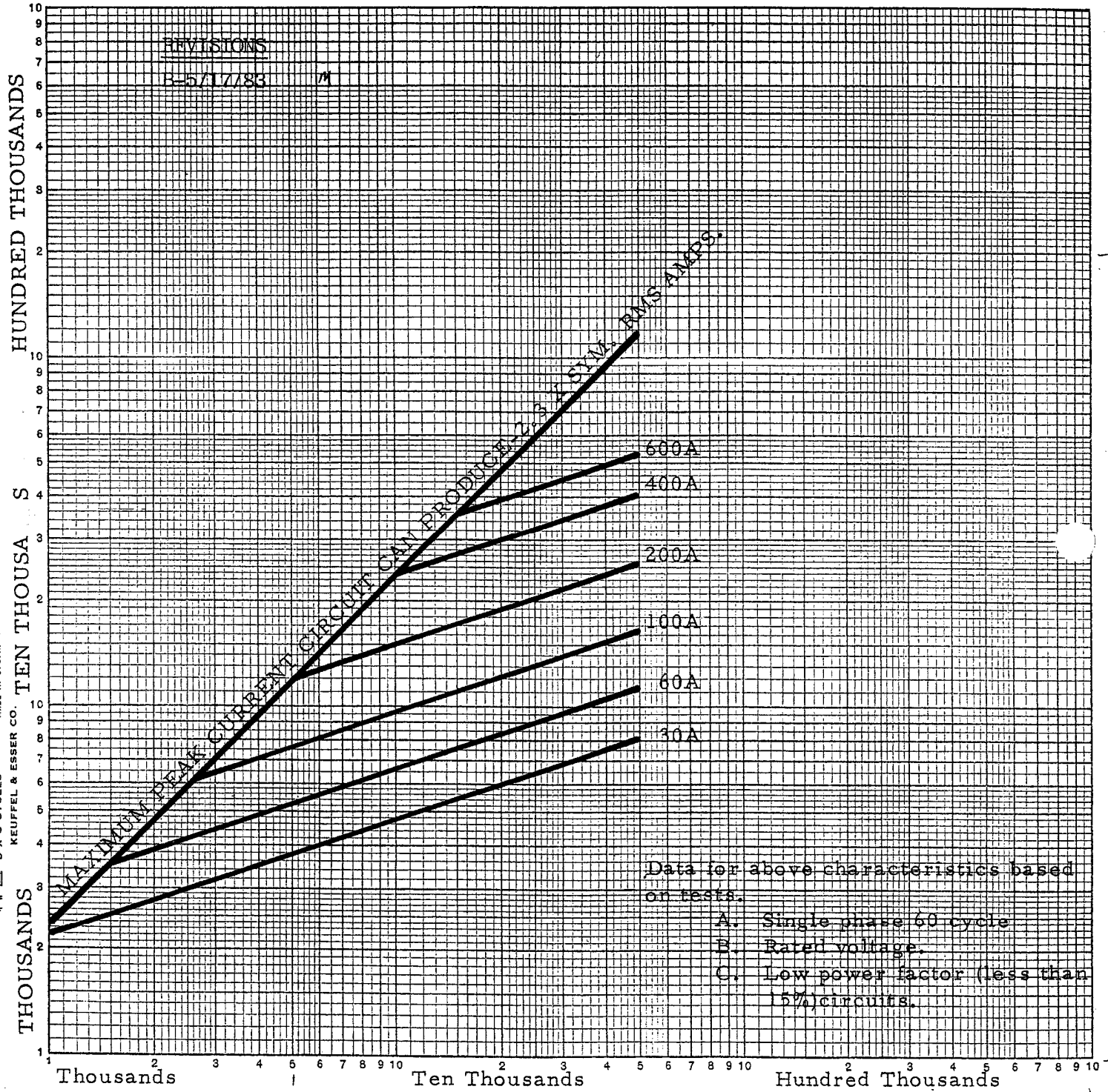
AVAILABLE CURRENT IN RMS SYMMETRICAL AMPERES
