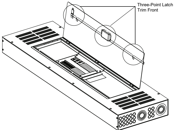
Figure 11: Three-Point Latch Trim Front
