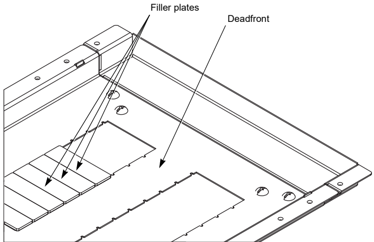
Figure 6: Deadfront Diagram
