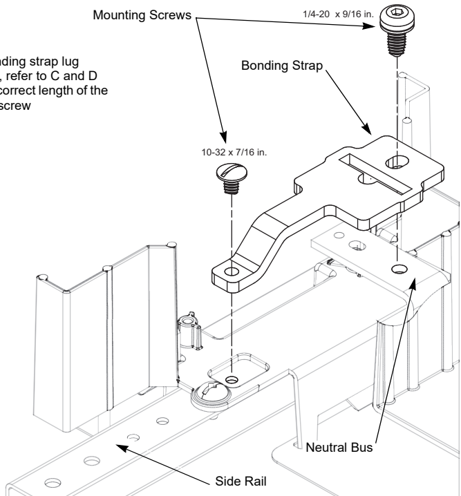
Figure 2: Bonding Strap Installation— 100 or 250 A Maximum NQ Panelboards
