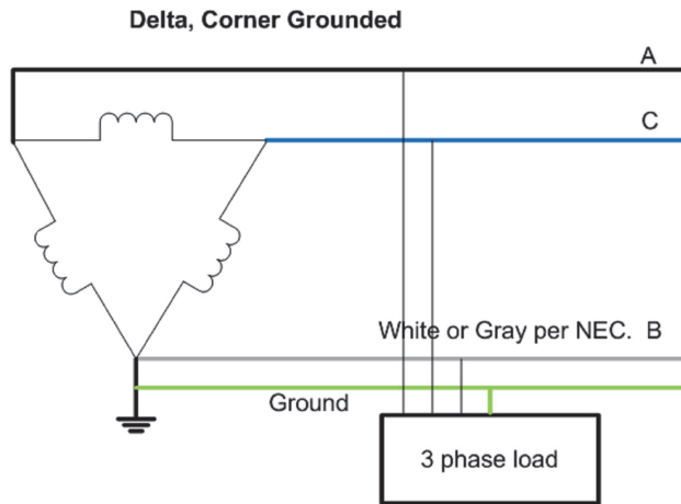
Figure 7: Corner Grounded Delta
