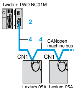
Connection to Lexium 05A via spring terminals (CN1)
