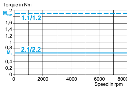
400/480 V 3-phase
