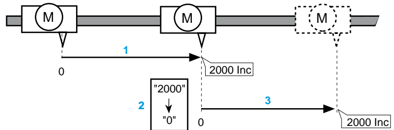
Positioning by 4000 increments with position setting
