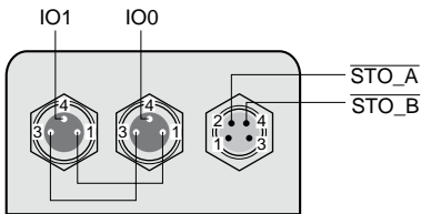
Insert for two I/O signals and STO signals for safety function
