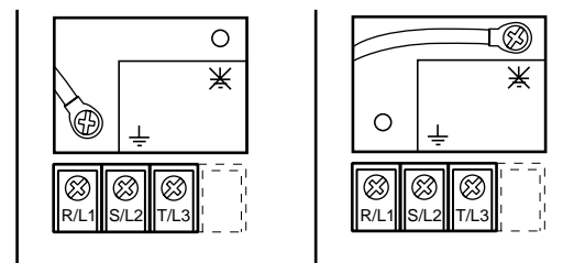
LXM 05●D57N4
