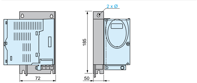
Mounting of the filter next to the stepper motor drive
