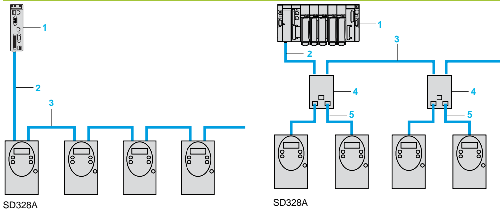
CANopen MotionBus connection
