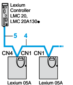
Connection to the CANopen Motionbus
