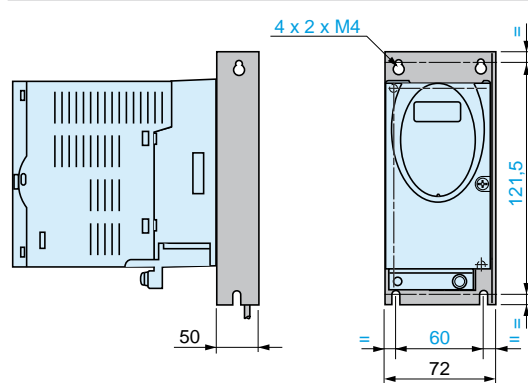
Mounting of the filter behind the stepper motor drive
