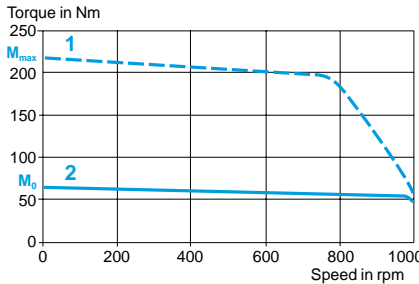
With LXM 15HC20N4X servo drive 230 V 3-phase
