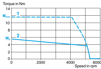
BSH 1002T servo motor With LXM 15LD28M3 servo drive 230 V 3-phase
