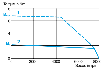
With LXM 05●D28M2 servo drive 230 V single-phase
