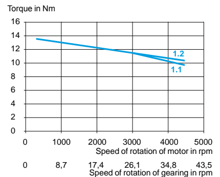
ILE2●661 with worm gear G8
