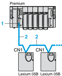
Connection to Lexium 05B via spring terminals (CN1)
