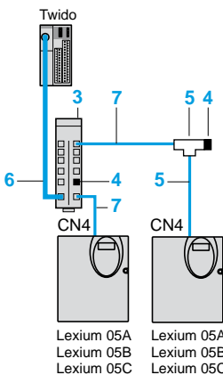
Connection to Lexium 05 via RJ45 connector (CN4)
