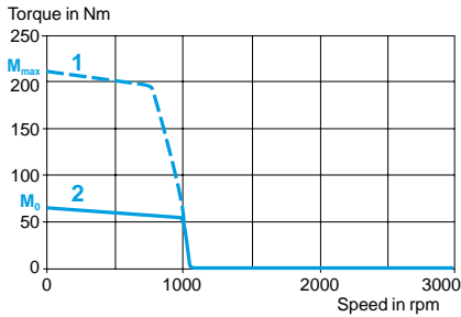
With LXM 15HC11N4X servo drive 230 V 3-phase
