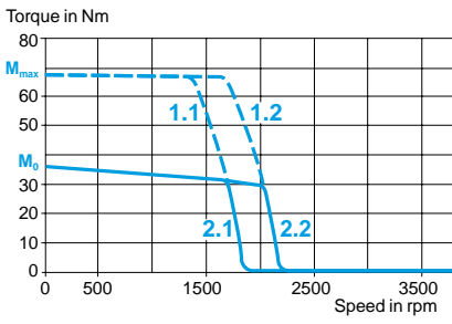
With LXM 15MD40N4 servo drive 400/480 V 3-phase
