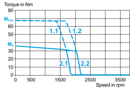
With LXM 15HC11N4X servo drive 400/480 V 3-phase
