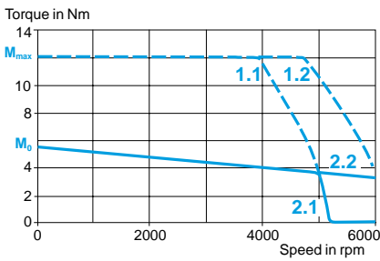
BSH 1002P servo motor With LXM 15LD17N4 servo drive 400/480 V 3-phase
