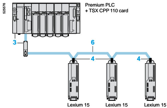
Example of connection to the CANopen machine bus via the AM0 2CA 001V000 adaptor 4
