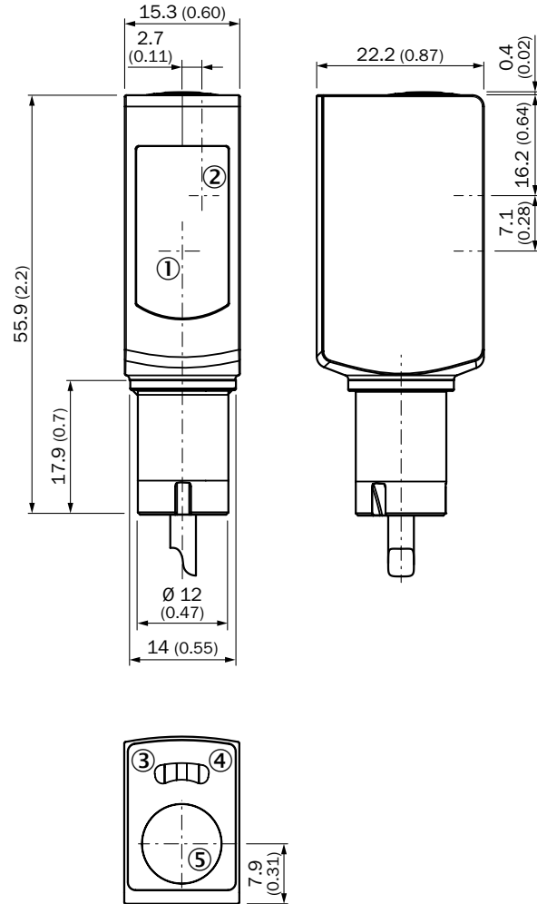
WTB4SL-3H, cable
