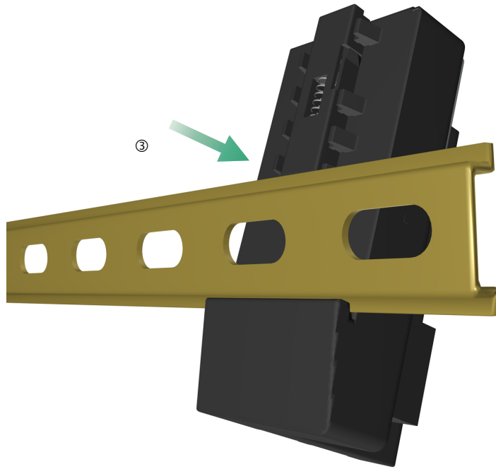
Fig. 304: Locating hook on the gateway
