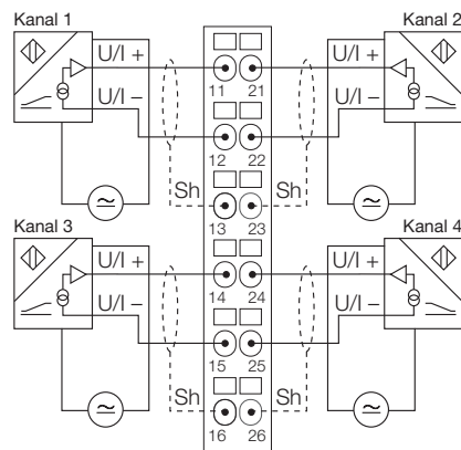
Fig. 145: 4-wire sensor with external sensor supply BL20-S6x-SBCSBC
