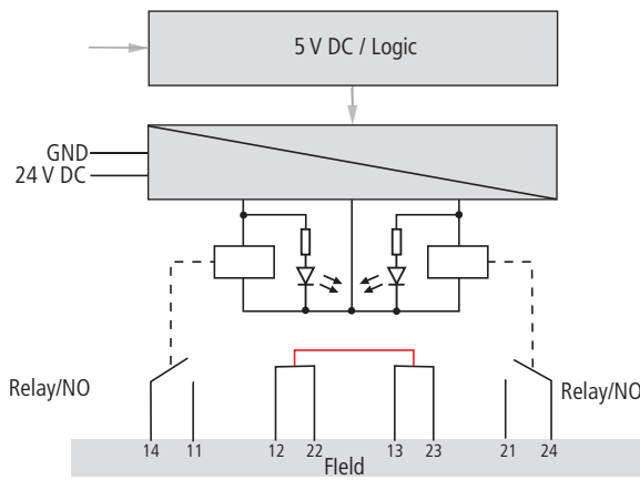
Fig. 236: Block diagram with base module BL20-S4x-SBBS
