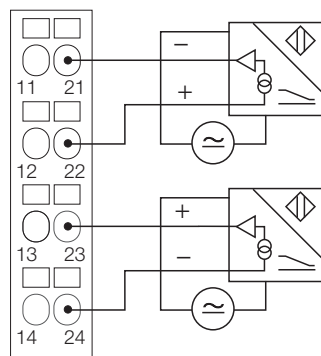
Fig. 155: Connection options with base module BL20-S4x-SBBS
