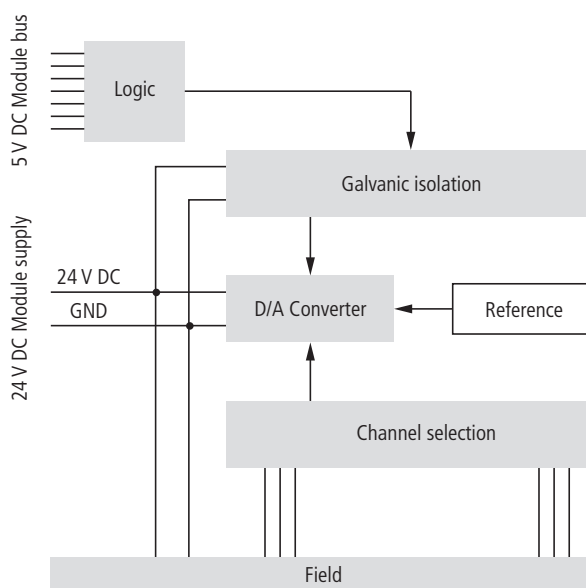
Fig. 131: Block Diagram
