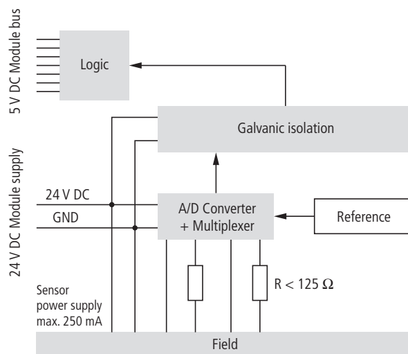
Fig. 109: Block Diagram
