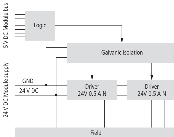
Fig. 166: Block Diagram
