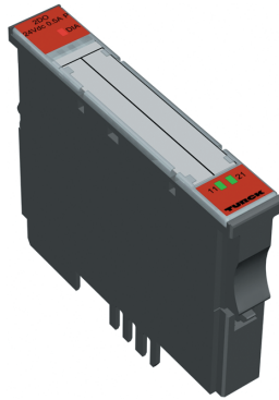
Fig. 159: BL20-2DO-24VDC-0.5A-P
