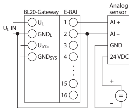
Fig. 150: 4-wire-sensor (U/I)
