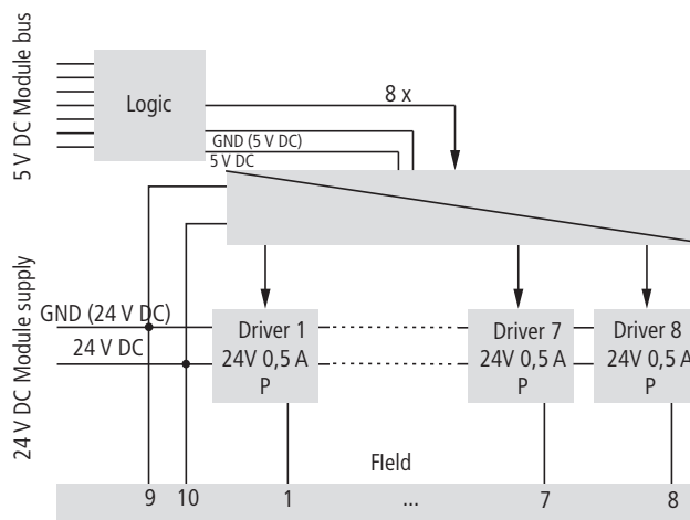
Fig. 186: Block Diagram
