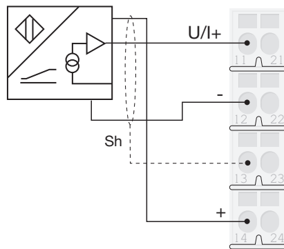
Fig. 105: 3-wire sensor with sensor supply via base module BL20-S4x-SBBS
