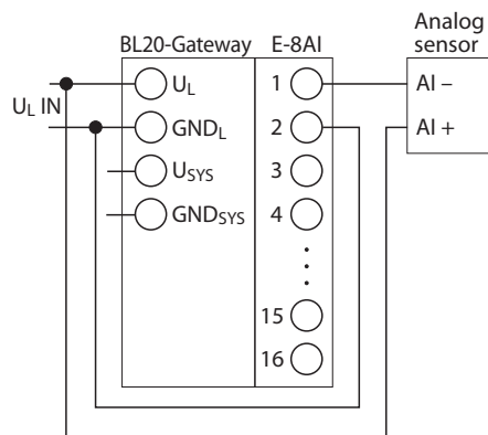
Fig. 151: 2-wire-sensor (U/I)
