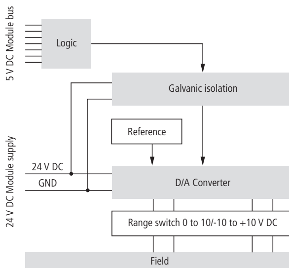
Fig. 216: Block Diagram
