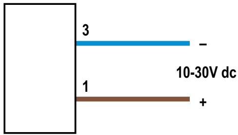
Figure 8. Emitter
