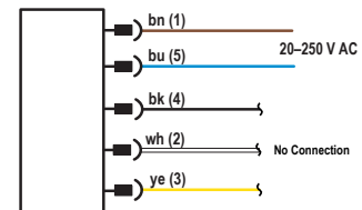
Figure 9. 5-pin 1/2"-20UNF QD emitters
