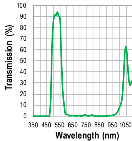
Figure 4. Percent transmission of light wavelengths through the FLTMG green filter
