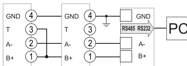
Fig. 22 M C BAC MS. RS485 seriel port.
