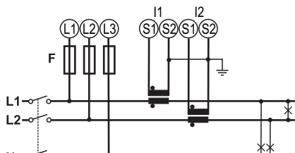
Fig. 13 Tofasesystem (3-leder), 2 CT. 315 mA sikring (F).
