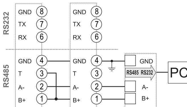
Fig. 20 M C 485232. RS485 seriel port.
