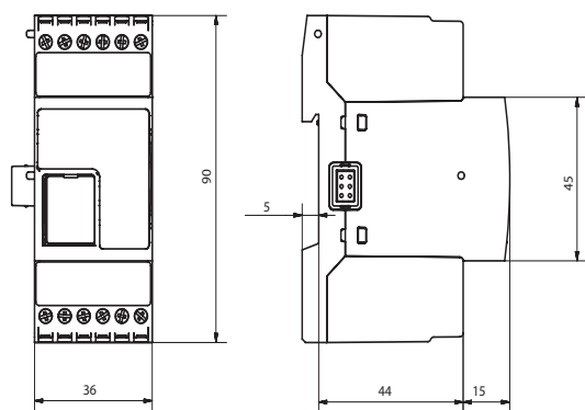
Fig. 3 Dimensions UWPM
