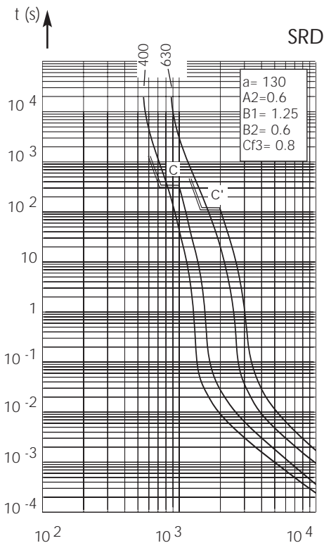
Above: Curves indicate, for each rated current, pre-arcing time vs. R.M.S. pre-arcing current.
