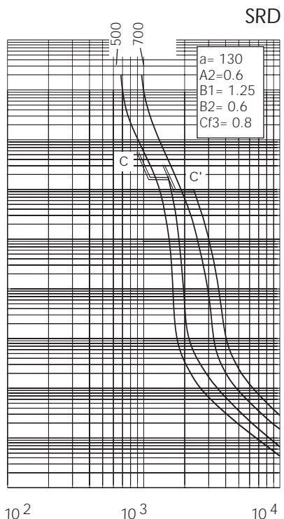
Above: Curves indicate, for each rated current, pre-arcing time vs. R.M.S. pre-arcing current.
