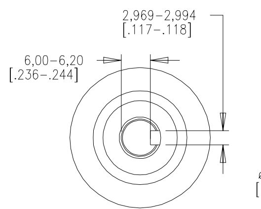
SHAFT DETAIL (NO SCALE)
