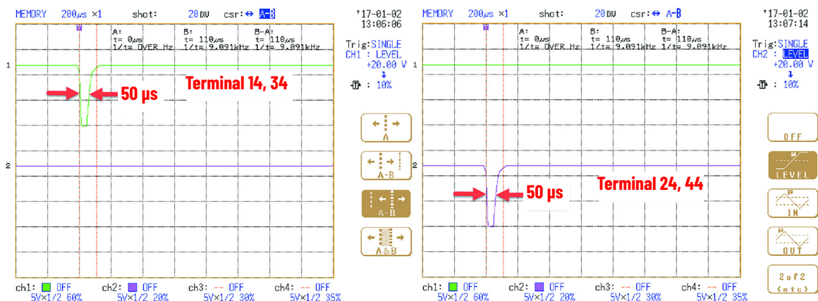
Figure 82 - OSSD Channel Transistor Test Pulse
