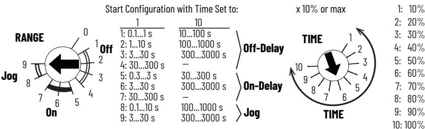
Figure 26 - EMD Safety Relay Range and Time
