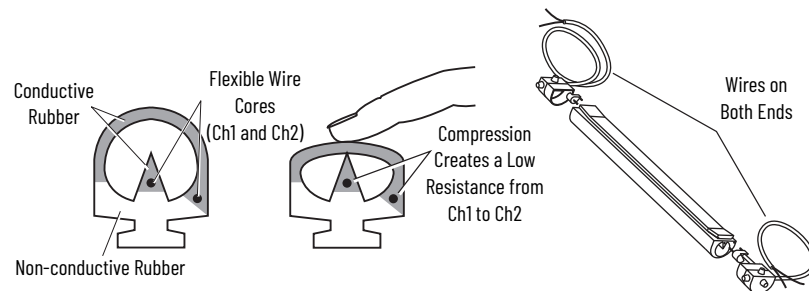
Figure 13 - Safedge Operating Principle
