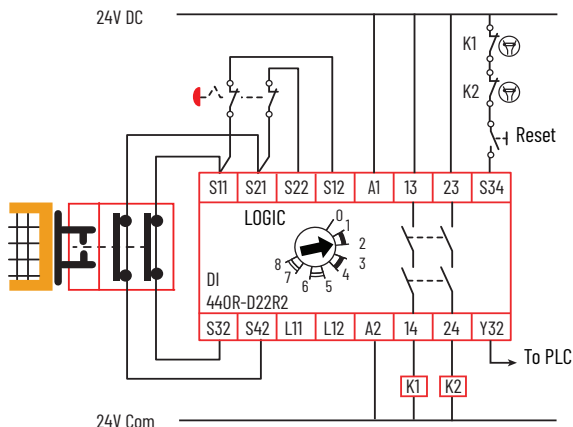
Figure 44 - With Two Devices with Mechanical Contacts and Monitored Manual Reset
