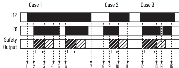
Figure 35 - Jog Timing Diagram
