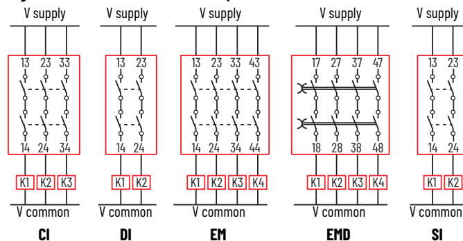
Figure 15 - Electromechanical Output Connections
