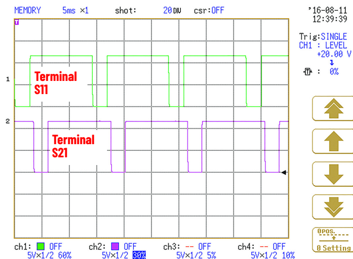
Figure 64 - CI Safety Relay Pulse Test Waveforms
