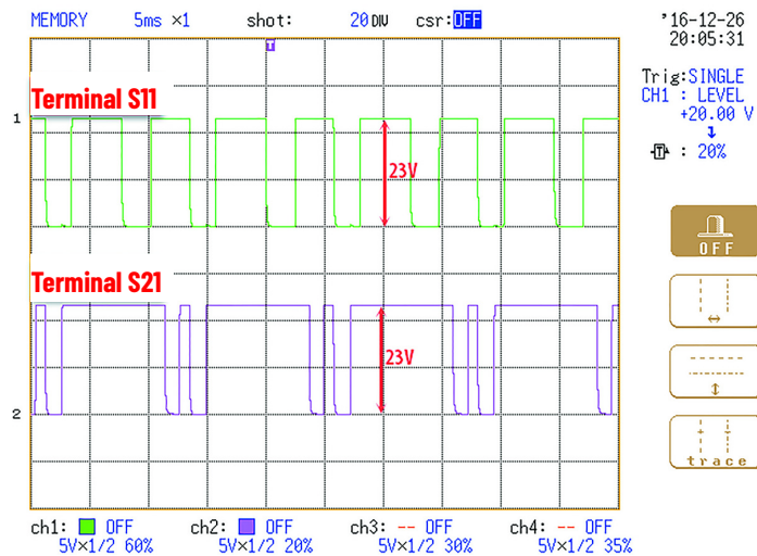
Figure 65 – DI, DIS, and SI Safety Relay Pulse Test Waveforms
