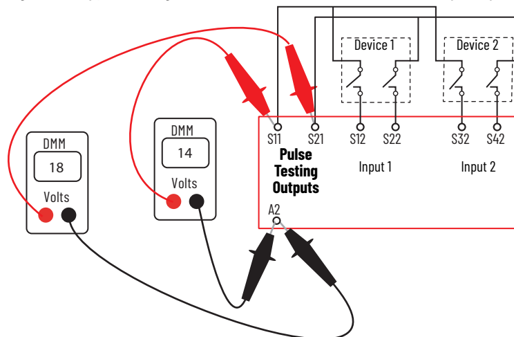
Figure 62 - Typical Voltage Measurements of the DI, DIS, and SI Safety Relays with Contacts Open
