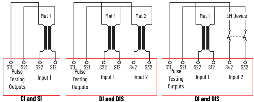
Figure 12 - Example Connections to Safety Mats
