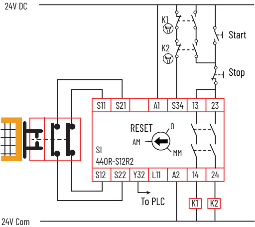
Figure 52 - SI Safety Relay Example
