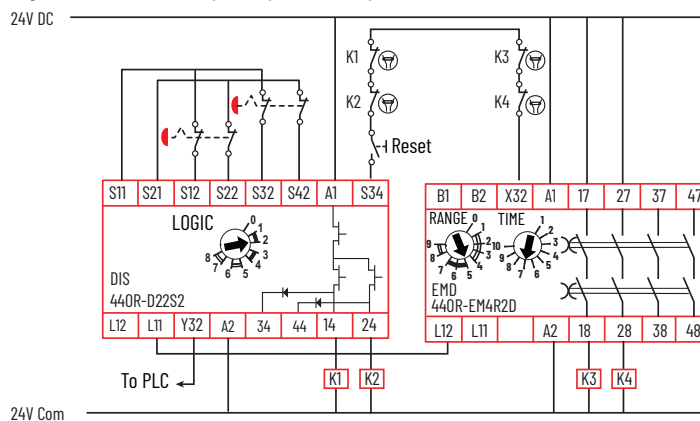
Figure 50 - EMD Safety Relay - On Delay
