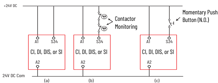
Figure 21 - Automatic/Manual Reset Connections
