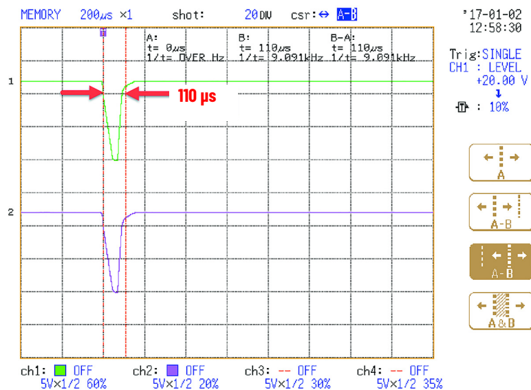
Figure 82 - OSSD Channel Transistor Test Pulse
