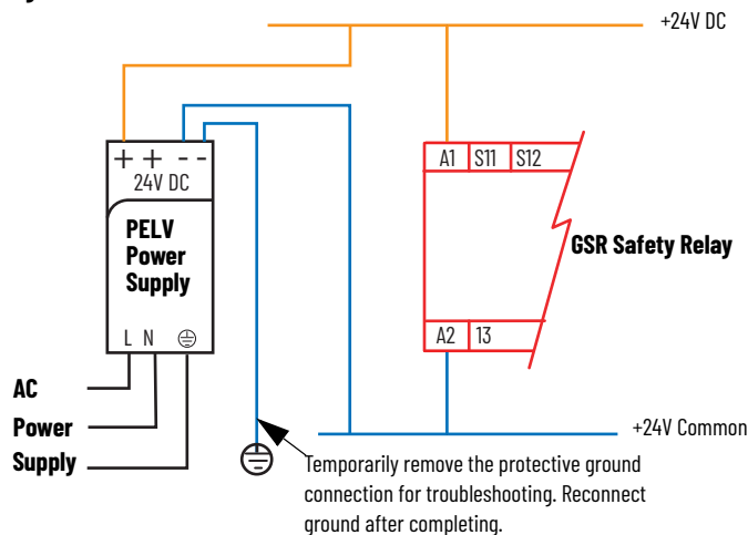
Figure 59 - 24V Common to Protective Earth Connection
