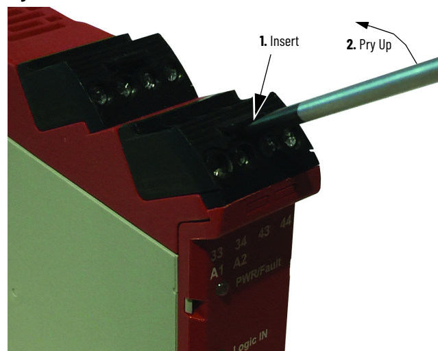
Figure 88 - Terminal Block Removal
