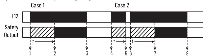
Figure 34 - On-delay Timing Diagram
