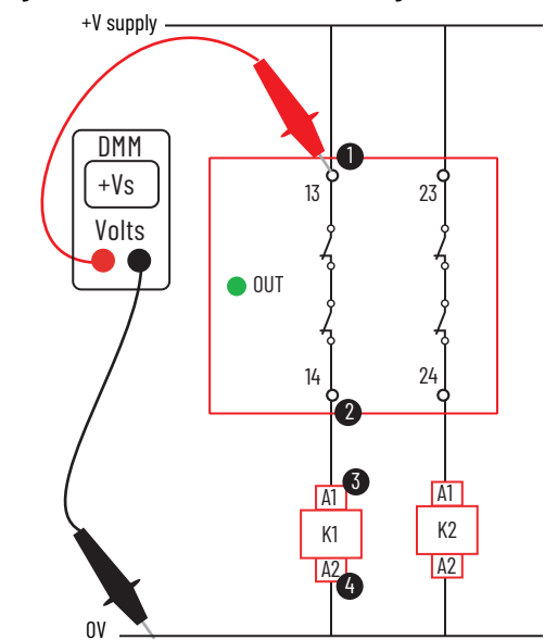
Figure 76 - Measure the Terminal Voltage
