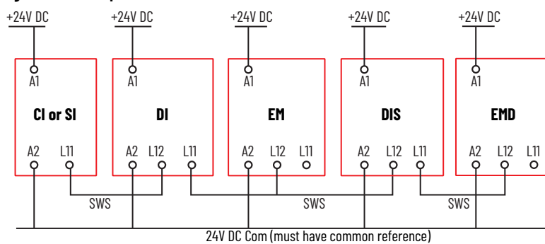
Figure 71 - Example SWS Connections
