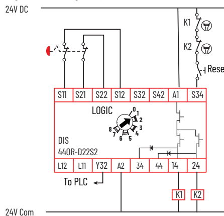
Figure 46 - Single Input, Monitored Reset
