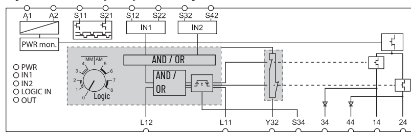
Figure 38 - DIS Safety Relay Circuit Diagram
