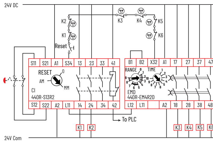
Figure 49 - EMD Safety Relay - Off Delay
