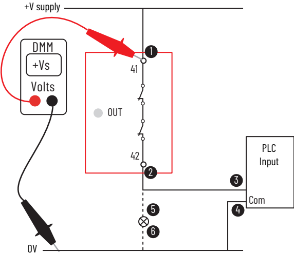
Figure 83 - Measure Voltage Aux Output Terminals
