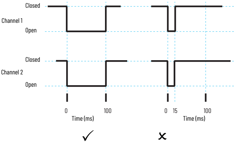
Figure 70 - Recovery Time
