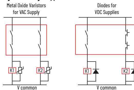
Figure 17 - Surge Suppressors
