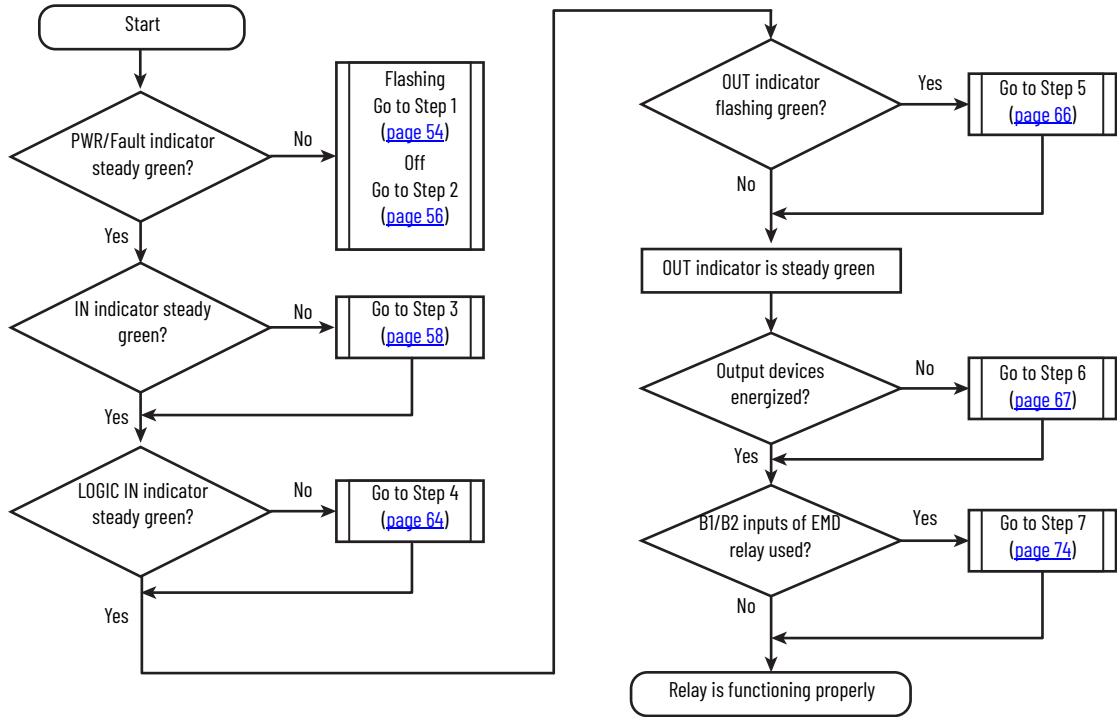
Figure 56 - Troubleshooting Flowchart
