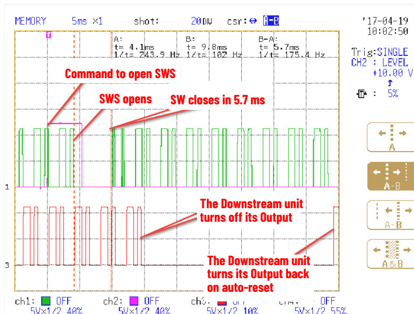
Figure 73 - Momentary Interruption of SWS Input
