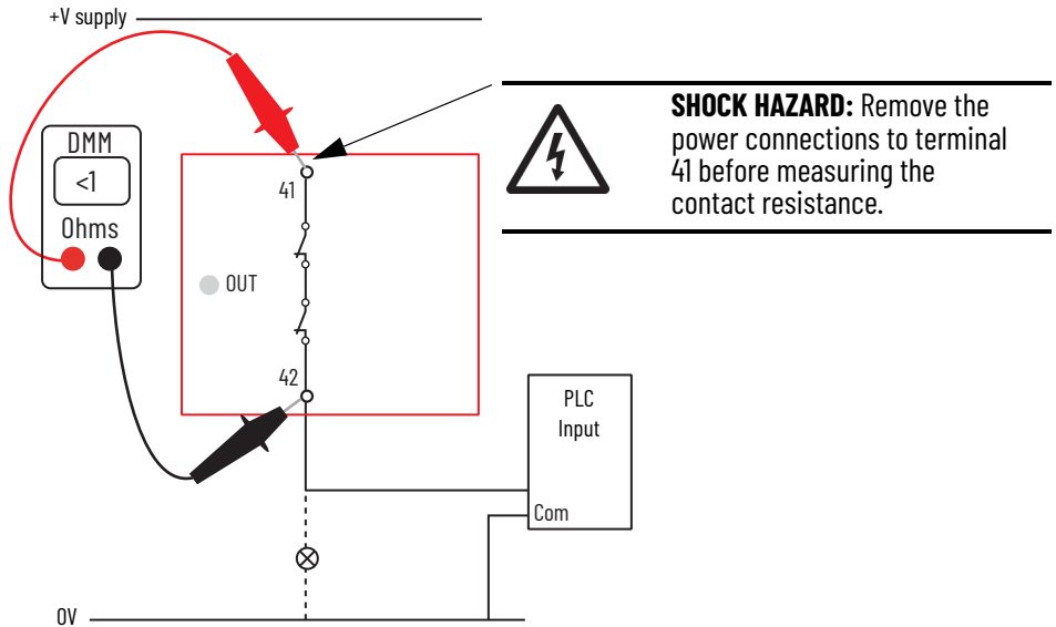
Figure 84 - Measure Contact Resistance of Aux Output Terminals
