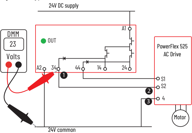
Figure 79 - Typical Connections to PowerFlex Drive
