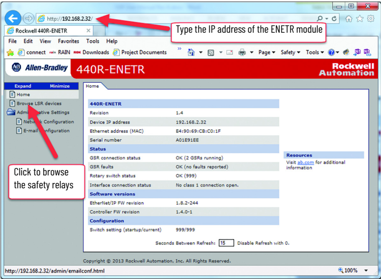
Figure 54 - ENETR Webpage
