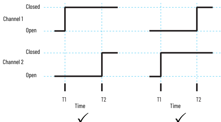
Figure 68 - GSR Safety Relays Have Infinite Simultaneity (Discrepancy)
