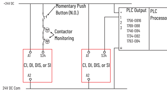
Figure 23 - Monitored Reset Connections
