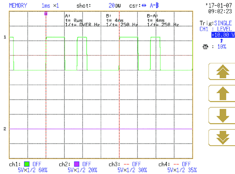
Figure 87 - The B1-B2 Waveform When the EMD Safety Relay Output is ON
