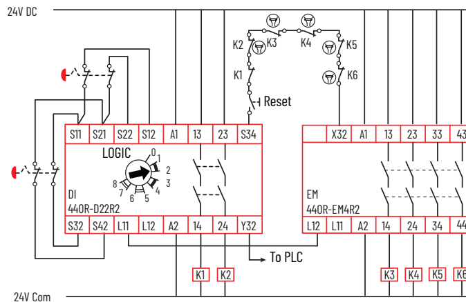
Figure 48 - Expansion of Immediate Safety Outputs
