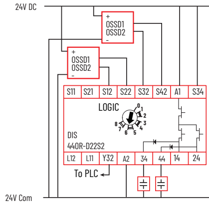
Figure 47 - High Capacitive Load
