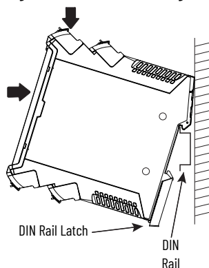
Figure 3 - DIN Rail Mounting
