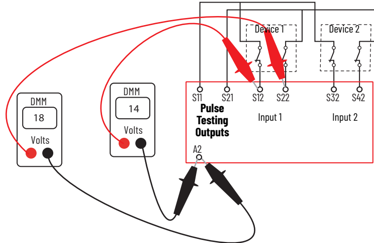
Figure 63 - Typical Voltage Measurements of the DI, DIS, and SI Safety Relays with Contacts Closed
