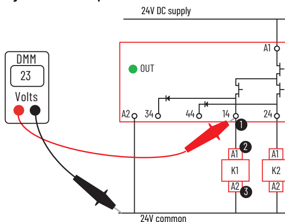
Figure 78 - OSSD Output Connections
