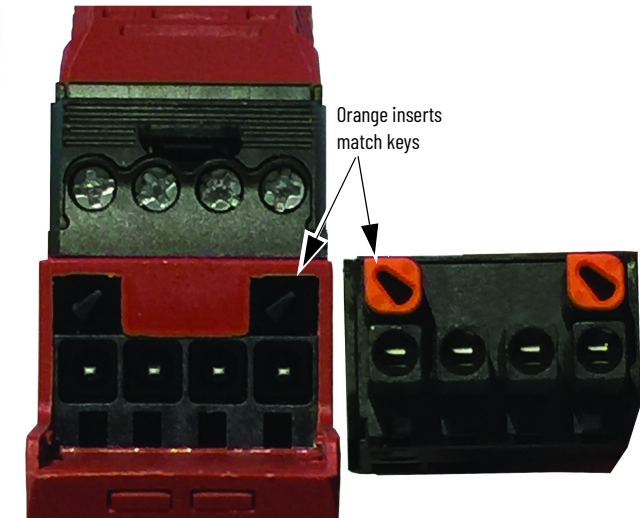
Figure 89 - Orange-colored Keyway
