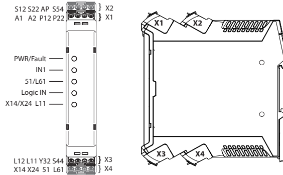
Figure 5 - Terminal Identification
