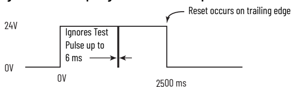
Figure 75 - Reset Input Ignores Test Pulses Up to 6 ms
