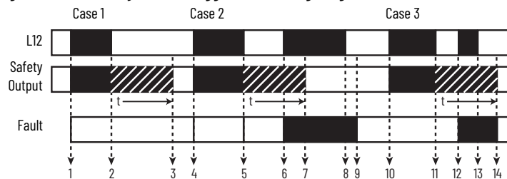
Figure 32 - Off-delay, Non-retriggerable Timing Diagram
