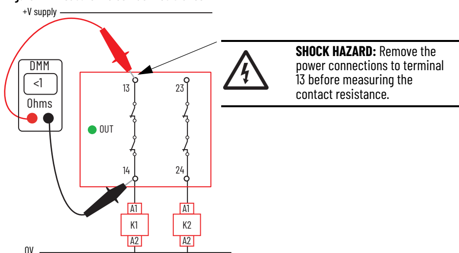
Figure 77 - Measure the Contact Resistance
