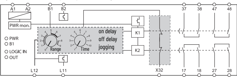
Figure 40 - EMD Safety Relay Circuit Diagram
