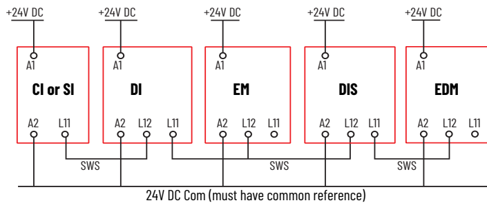
Figure 18 - Example SWS Connections
