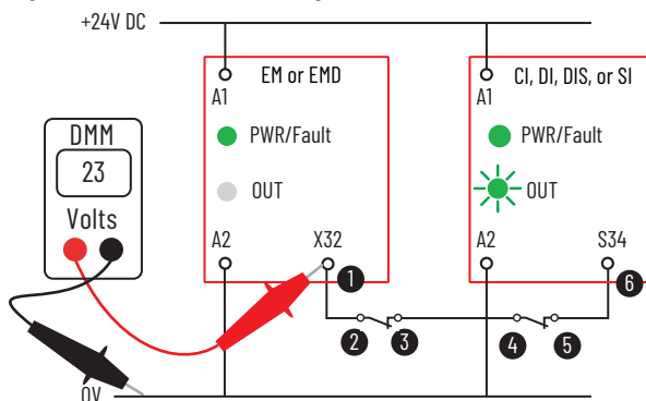
Figure 86 - Measure X32 Voltage
