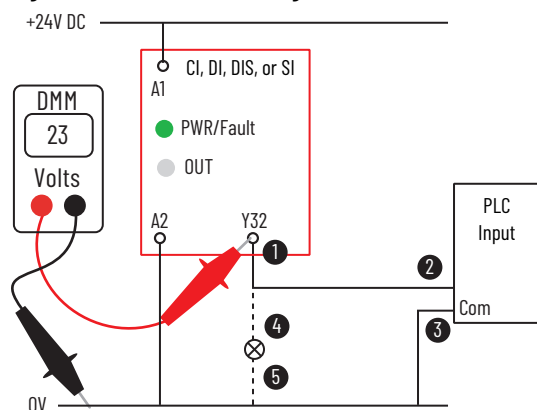
Figure 85 - Measure Y32 Voltage
