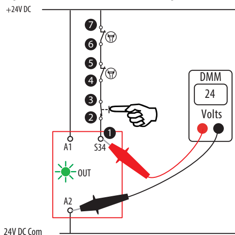
Figure 74 - Measure Reset/Monitoring Circuit Voltage
