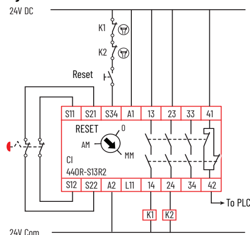
Figure 42 - Mechanical Contacts with Monitored Manual Reset
