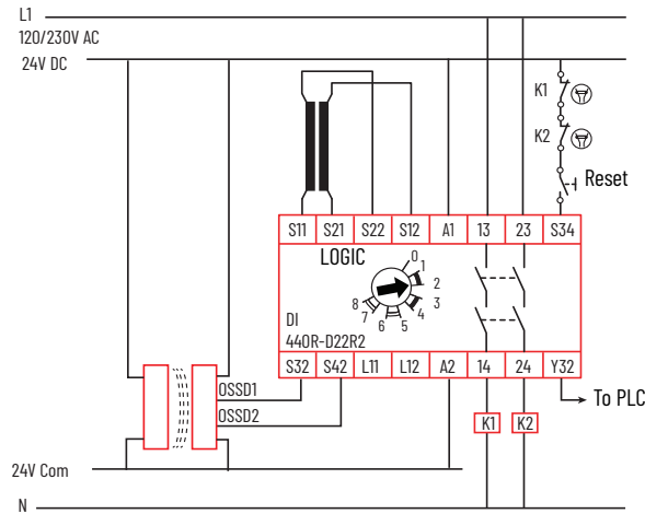
Figure 45 - With a Safety Mat and Device with OSSD Outputs, Monitored Manual Reset, AC Loads
