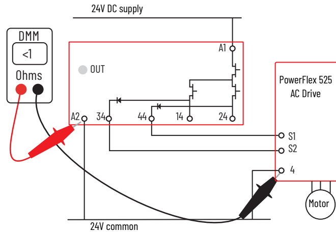
Figure 80 - Continuity Test of the Voltage Supply Common Connection
