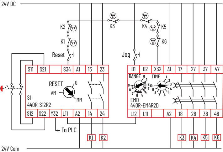
Figure 51 - EMD Safety Relay - Jog
