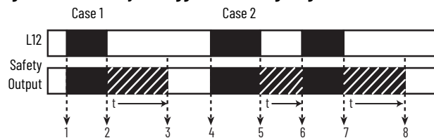
Figure 33 - Off-delay, Retriggerable Timing Diagram
