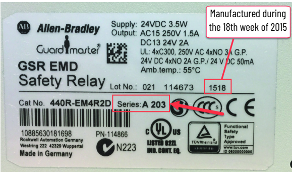
Figure 90 - Product Label - Series and Revision Identification
