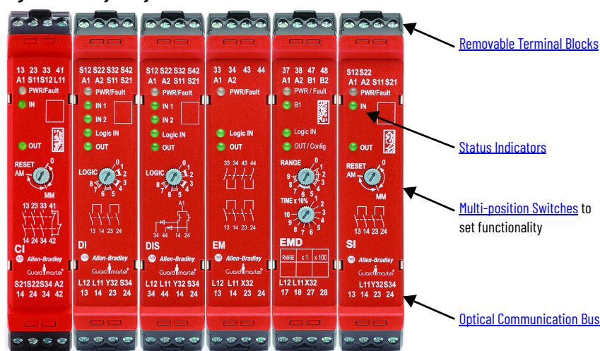
Figure 1 - Safety Relays
