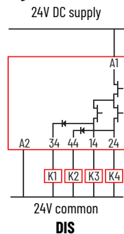
Figure 16 - OSSD Output Connections
