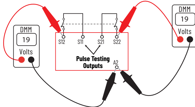
Figure 61 - Check the CI Safety Inputs with the Device Contacts Closed
