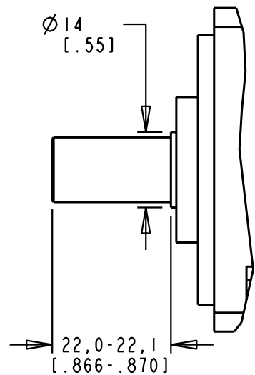
SHAFT DETAIL (NO SCALE)
