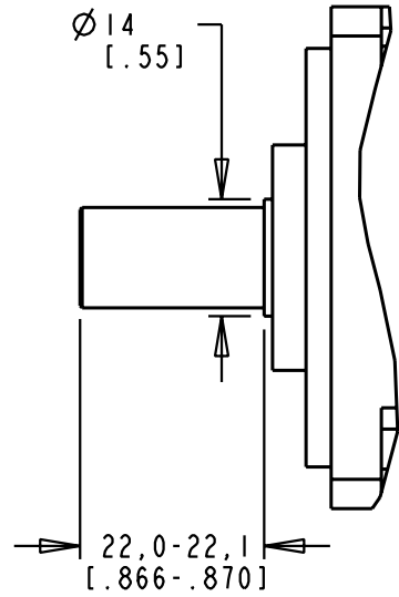
SHAFT DETAIL (NO SCALE)
