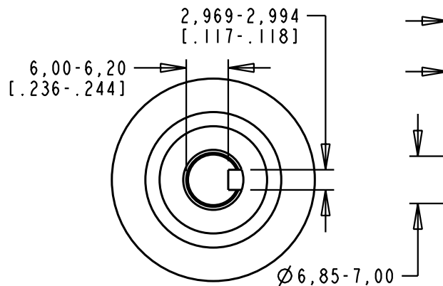
SHAFT DETAIL (NO SCALE)
