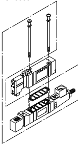
SV3000-M1-□
