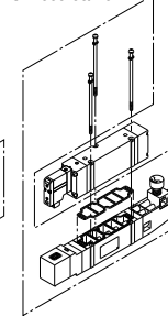
SV4000-00/N0-□
