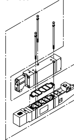
SV4000-M1-□
