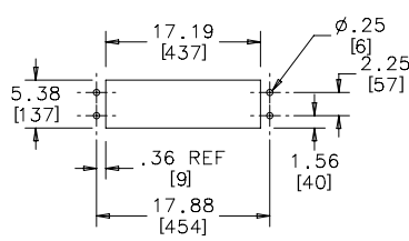
Blower Cutout
